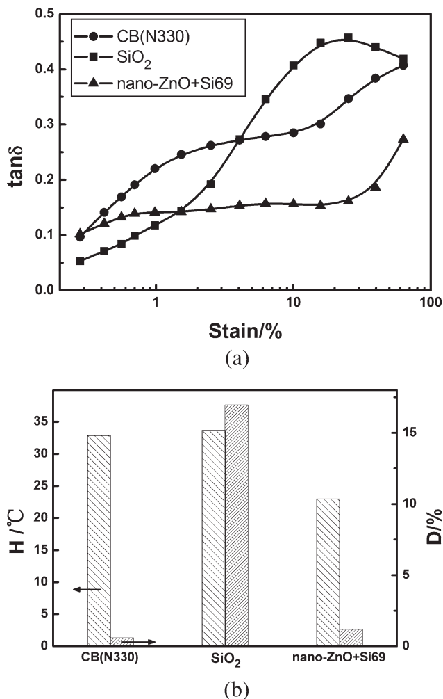
Figure 11 Comparison of dynamic mechanical properties among composites compounded with nano-ZnO and traditional reinforcing fillers: (a) \tan\delta ; (b) compression fatigue properties. H represents the compression heat build-up and D represents the difference between ultimate compression deformation rate and initial one.
