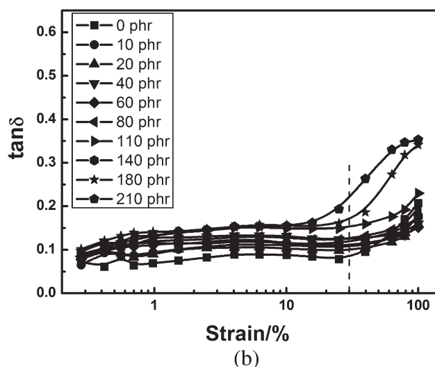
Figure 9 Influence of in-situ modification on \tan\delta of nano-ZnO filled composites as a function of the filler loading: (a) untreated nano-ZnO filled composites; (b) in-situ modified nano-ZnO filled composites.
