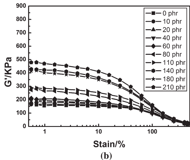
Figure 4 Payne effect of nano-ZnO filled gross rubber: (a) untreated nano-ZnO filled composites; (b) in-situ modified nano-ZnO filled composites.
